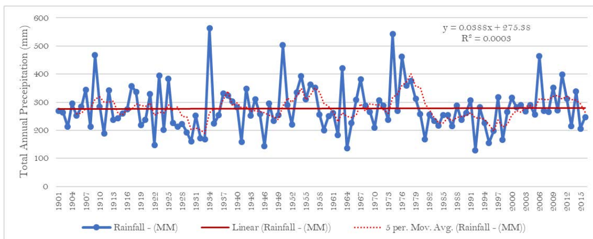
Figure 4.7 - Historical trend in annual precipitation in Namibia (1901 - 2016)
