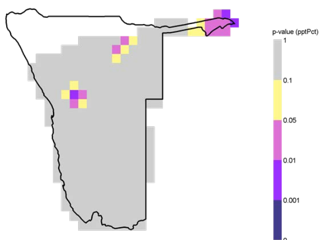
Figure 4.8 - Statistical confidence of precipitation changes (1901 - 2016)
