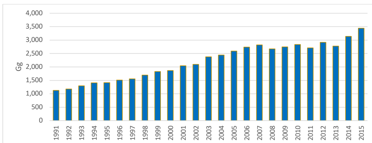
Figure 4.3- Evolution of CO 2 emissions (Gg) in the Energy Sector (1991 - 2015)
