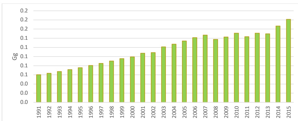
Figure 4.5- Evolution of N 2 O emissions (Gg) in the Energy Sector (1991 - 2015)
