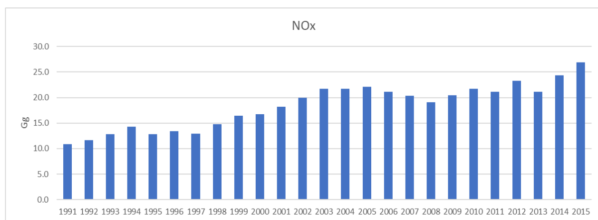
Figure 4.6- Evolution of NO x emissions (Gg) in the Energy Sector (1991 - 2015)
