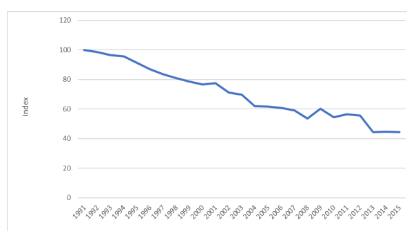
Figure 3.3 - GDP emissions index (1991 - 2015)
