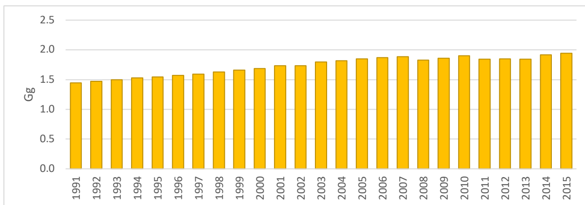
Figure 4.4- Evolution of CH 4 emissions (Gg) in the Energy Sector (1991 - 2015)
