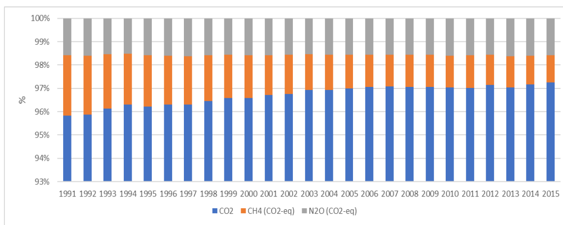
Figure 4.2- Share of emissions by gas (%) for the Energy sector (1991 - 2015)
