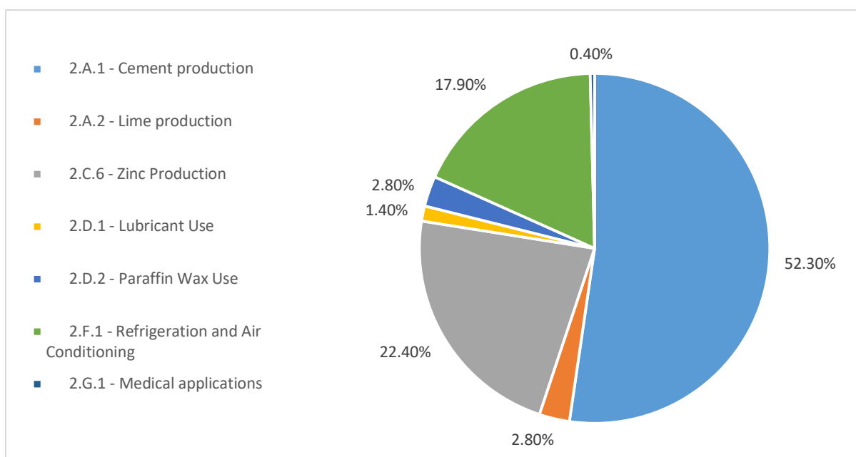
Figure 5.1- Percentage distribution of emissions for IPPU Sector (2015)
