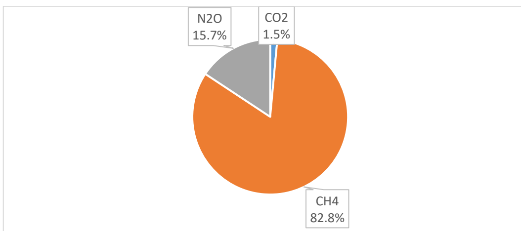
Figure 7.1- Percentage distribution of emissions for waste Sector (2015)
