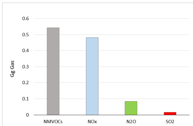
Figure 7.2- Emissions of N 2 O, NO x , NMVOCs and SO 2 from waste Sector (2015)
