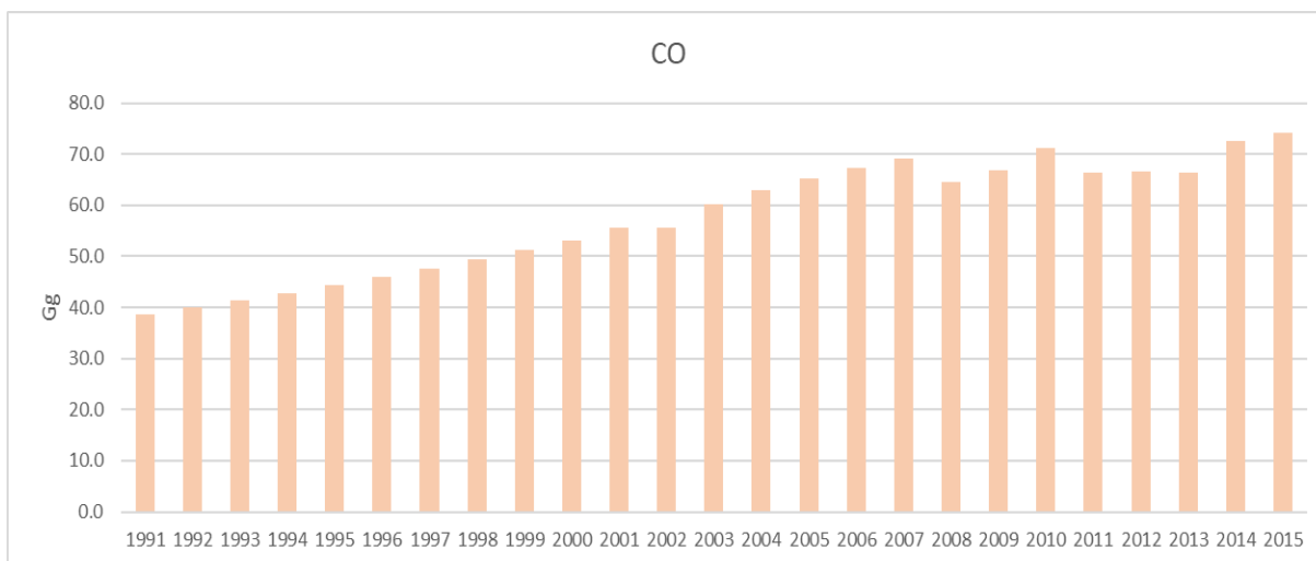
Figure 4.7- Evolution of CO emissions (Gg) in the Energy Sector (1991 - 2015)
